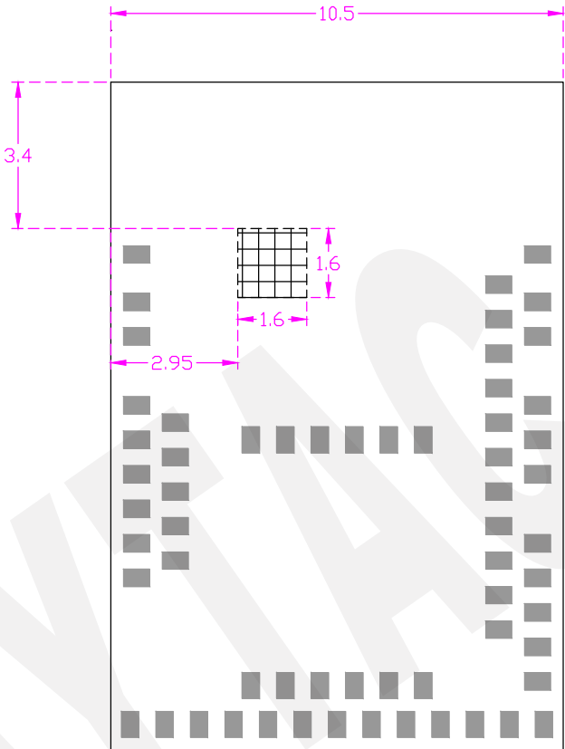
Top View (Unit: mm)
