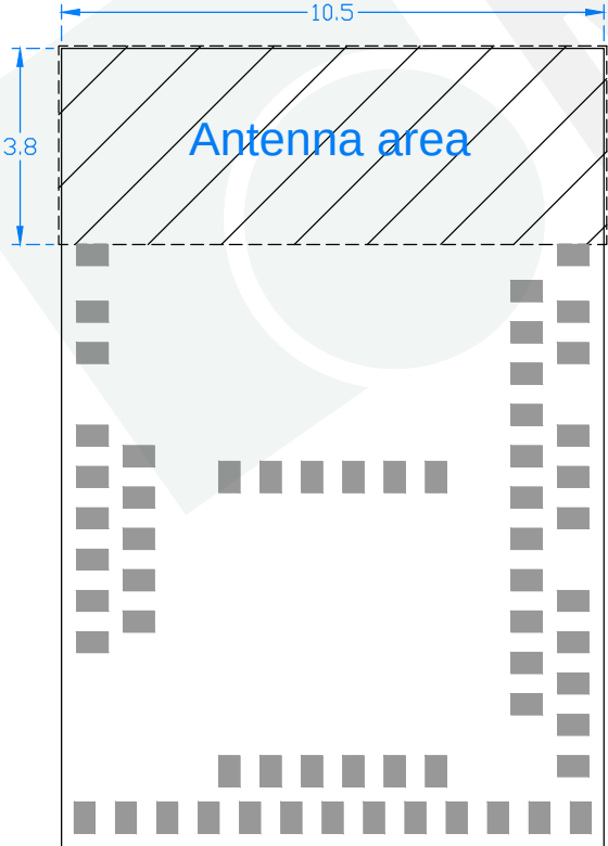
Top View (Unit: mm)
