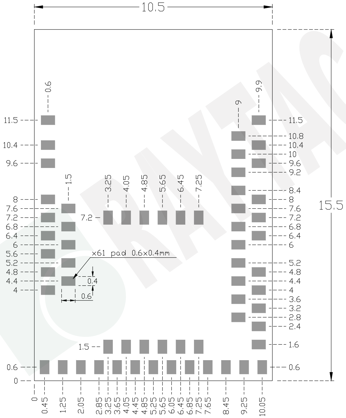
Top View (Unit: mm)
