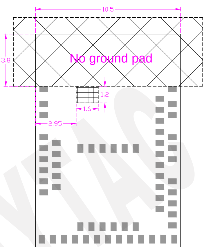
Top View (Unit: mm)
